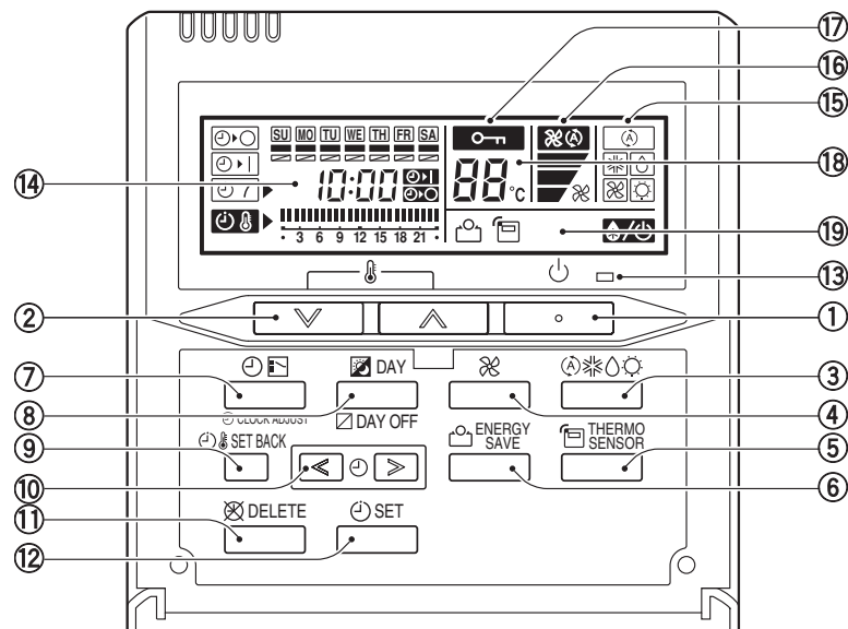
Fig. 3 Remote controller
