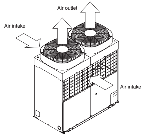
Fig. 2 Outdoor Unit
