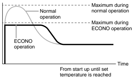
Running current and power consumption
